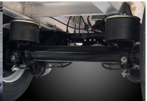
Hendrickson Intraax® suspension; All steel parts finished with Corsol® WB Corrosion Protection.
